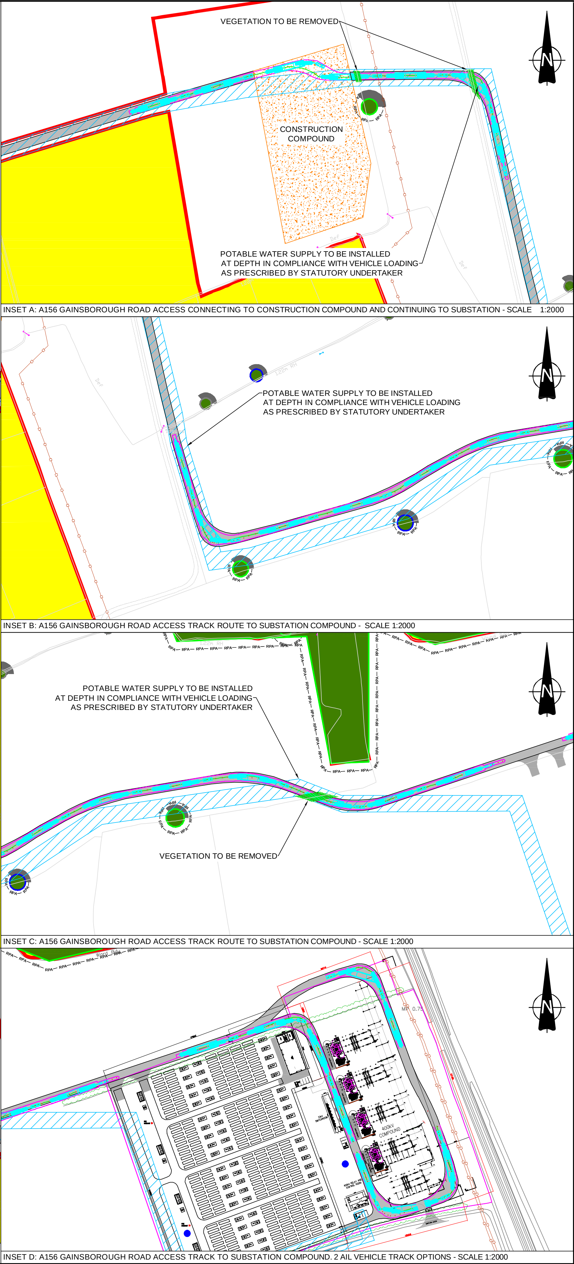
INSET D: A156 GAINSBOROUGH ROAD ACCESS TRACK TO SUBSTATION COMPOUND. 2 AIL VEHICLE TRACK OPTIONS - SCALE 1:2000
